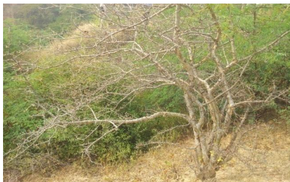
Fig.1. Guggal plant
