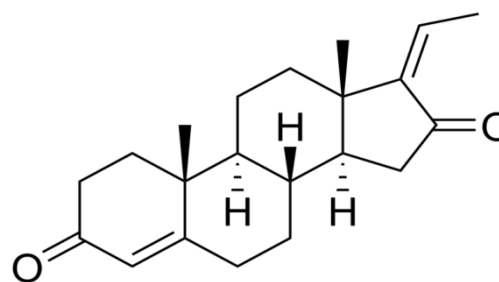
Fig.4 Guggulsterone - Z
