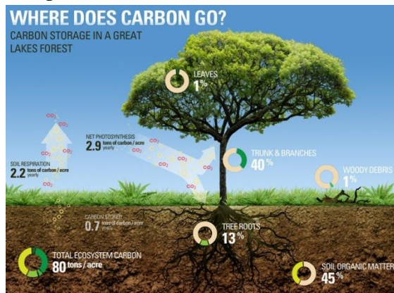
Figure 1: Forest carbon pools
